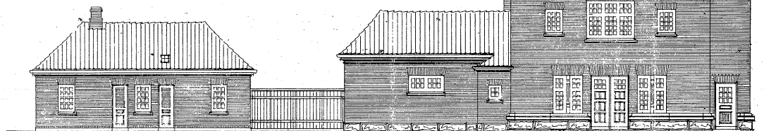
FACADE MOD NORD.
