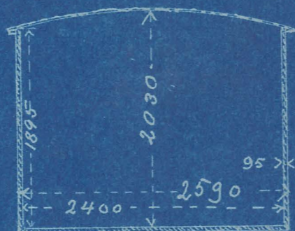
Snit E-F.
