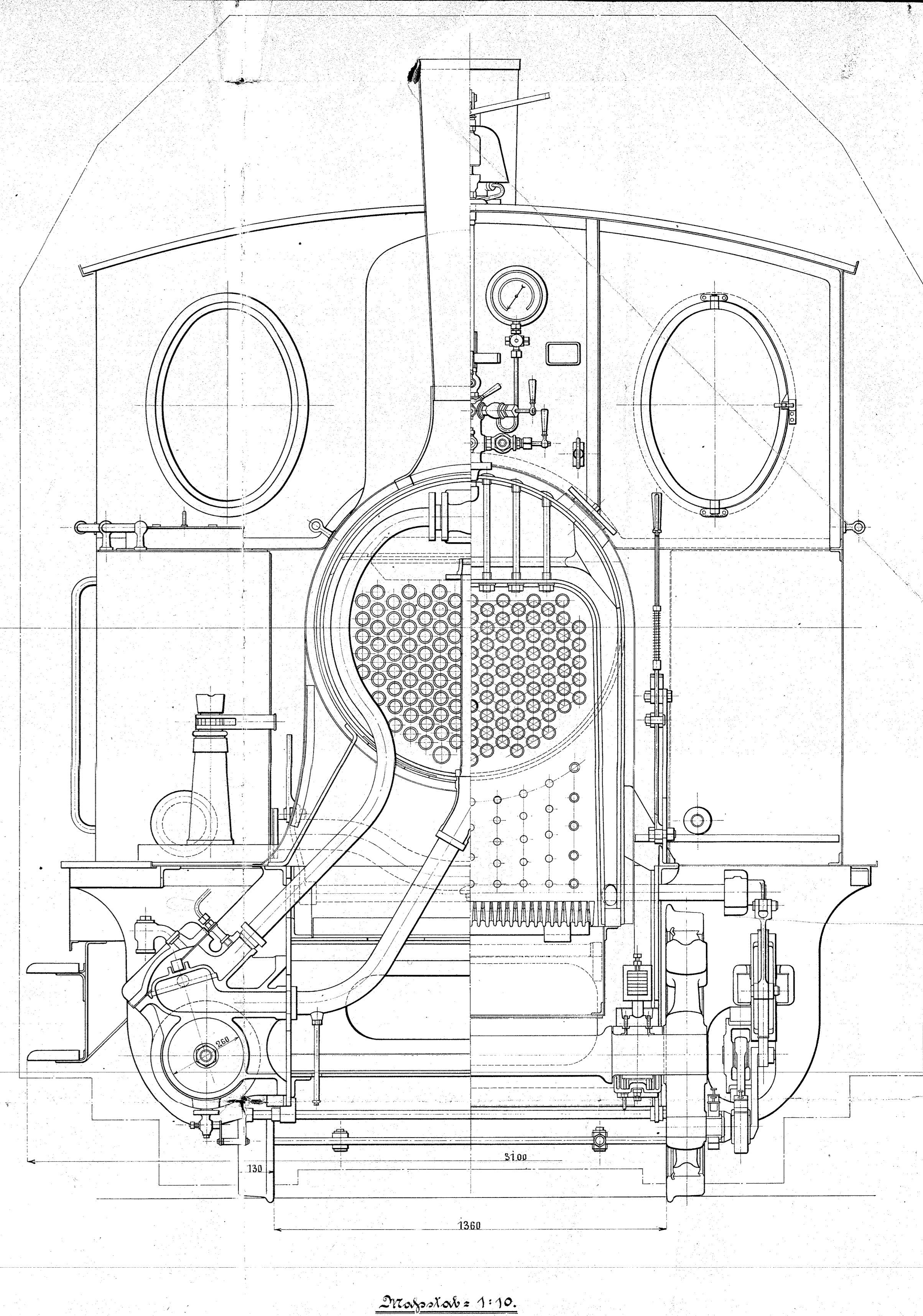
Detailabz. 1:10.
