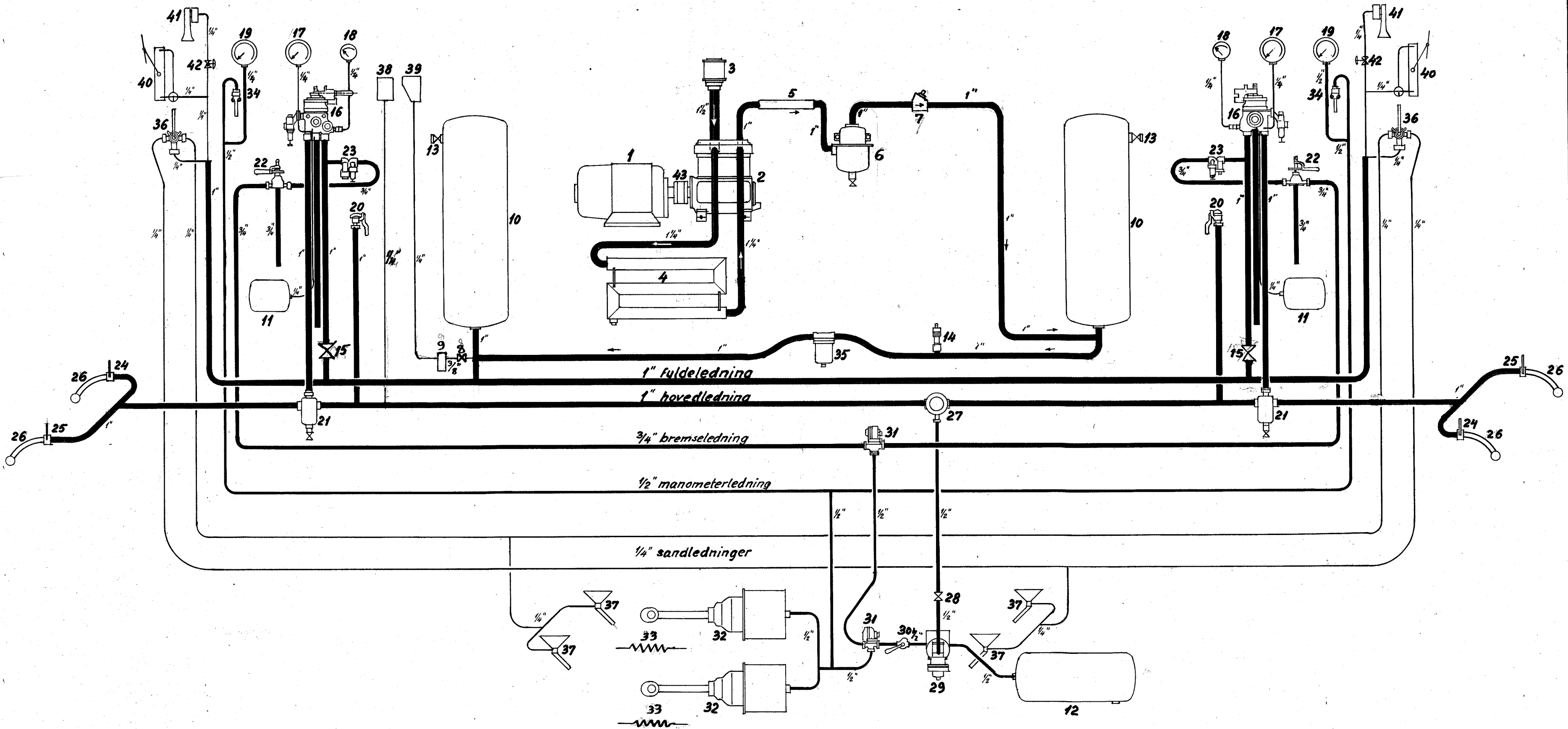
TRYKLIFT- RØRDIAGRAM ML 1208, 1209, 3202, 5203 AALBORG PRIVATBANER T.T.I. 9-11-51 W.B.
