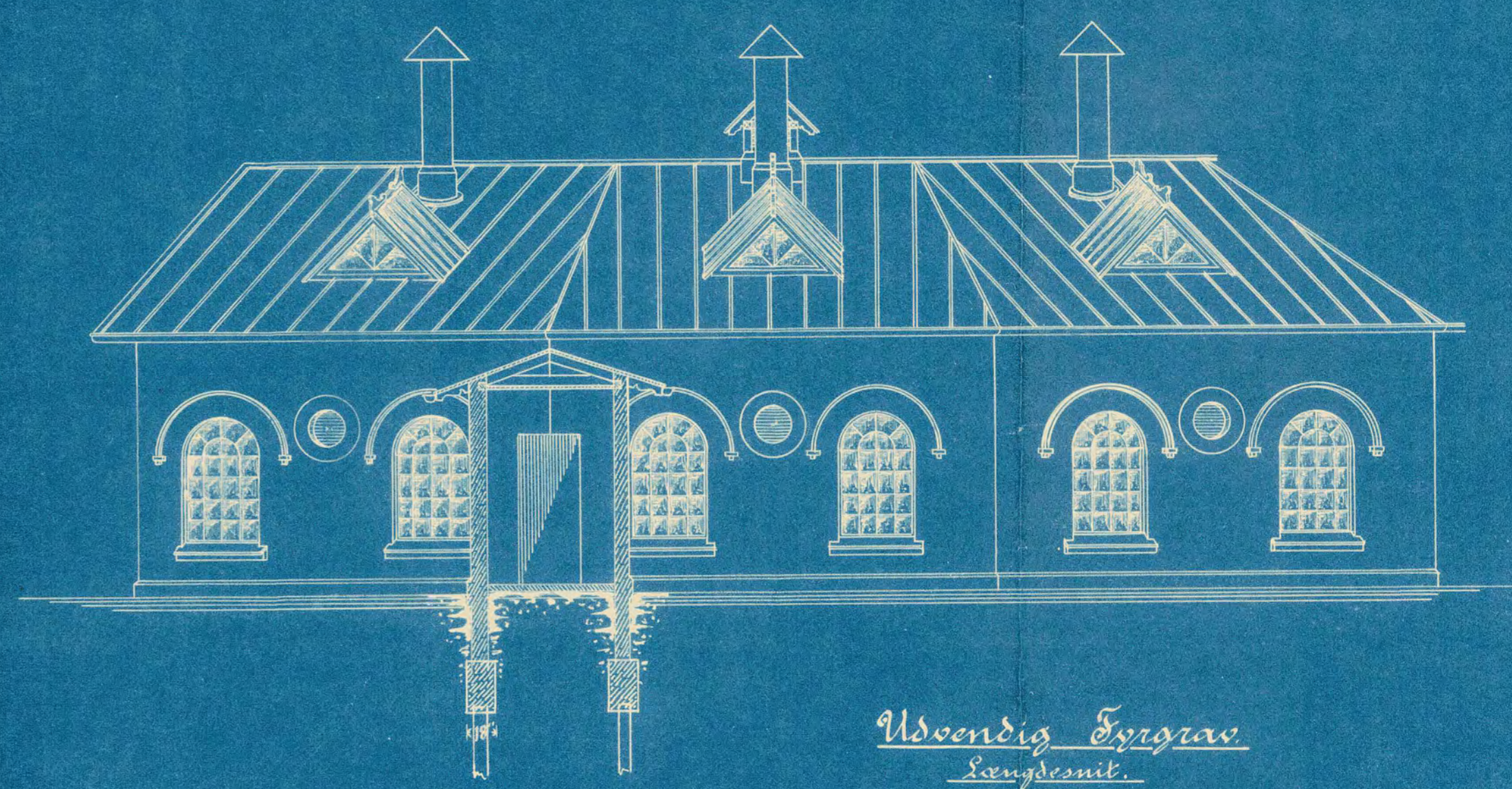
Bag-Facade.
