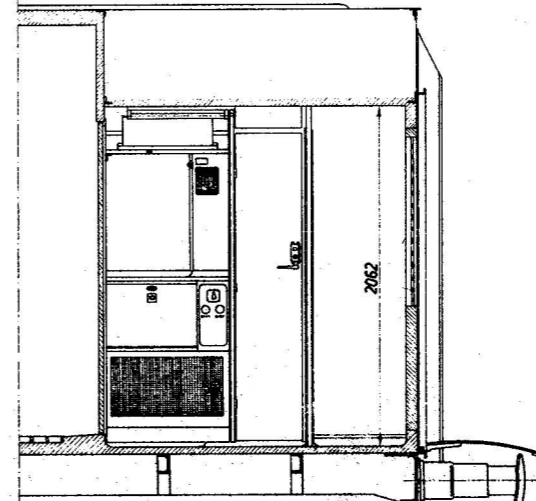
Snit D-D.
