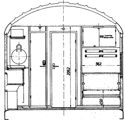
Snit C-C.
