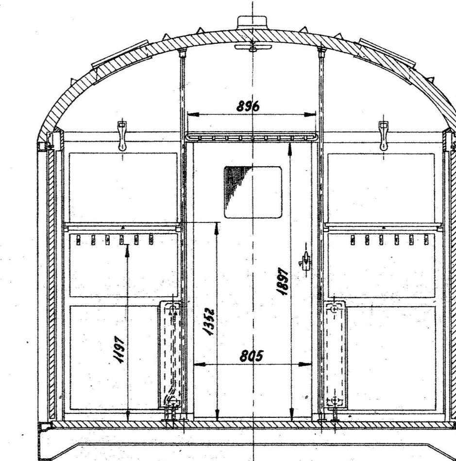
Snit F-F
