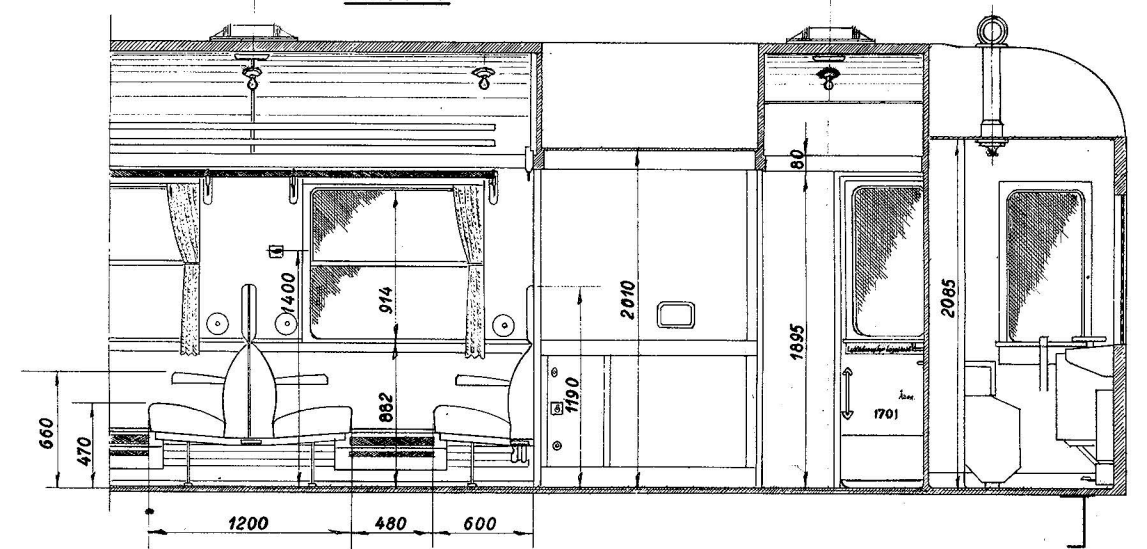
Snit f-f
