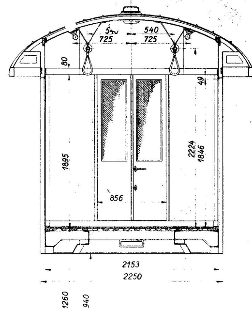
Snit-B-B
