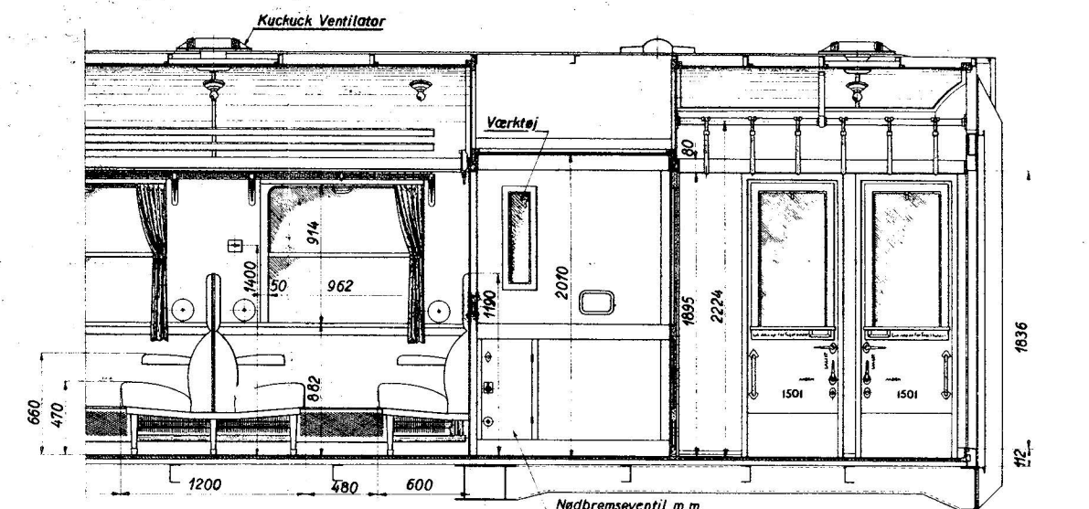
Snit-E-E
