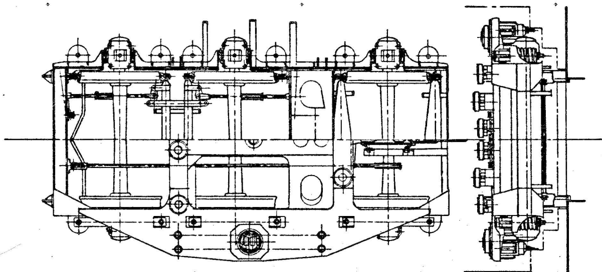
Maskinbogie
